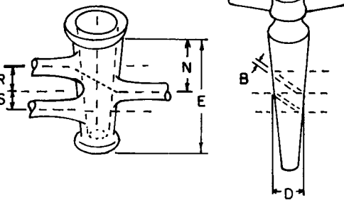
FIG. 3 Double Oblique-Bore (3-Way) Stopcock
